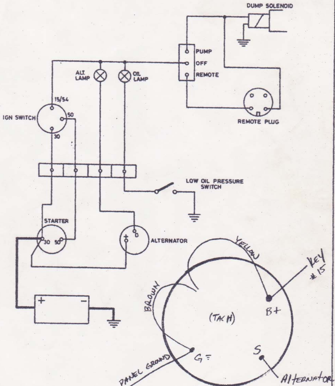
ELECTRICAL DIAGRAM - SIDEWINDER FULL DRESS AND ARIZONA SPECIAL Delco → R TERM.
