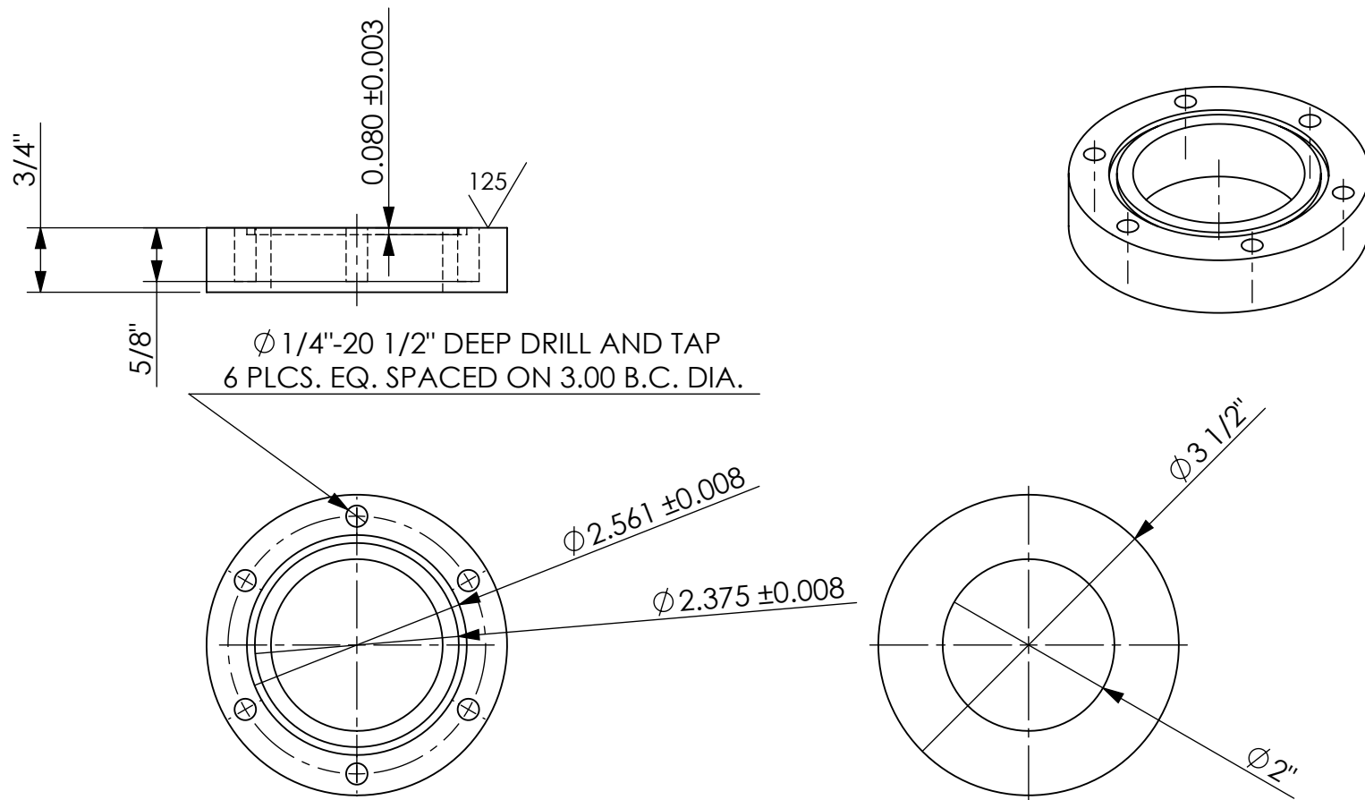
'O' RING #142
