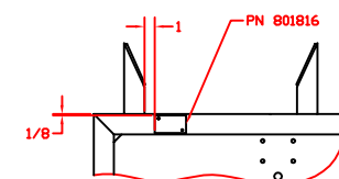
VIEW C
