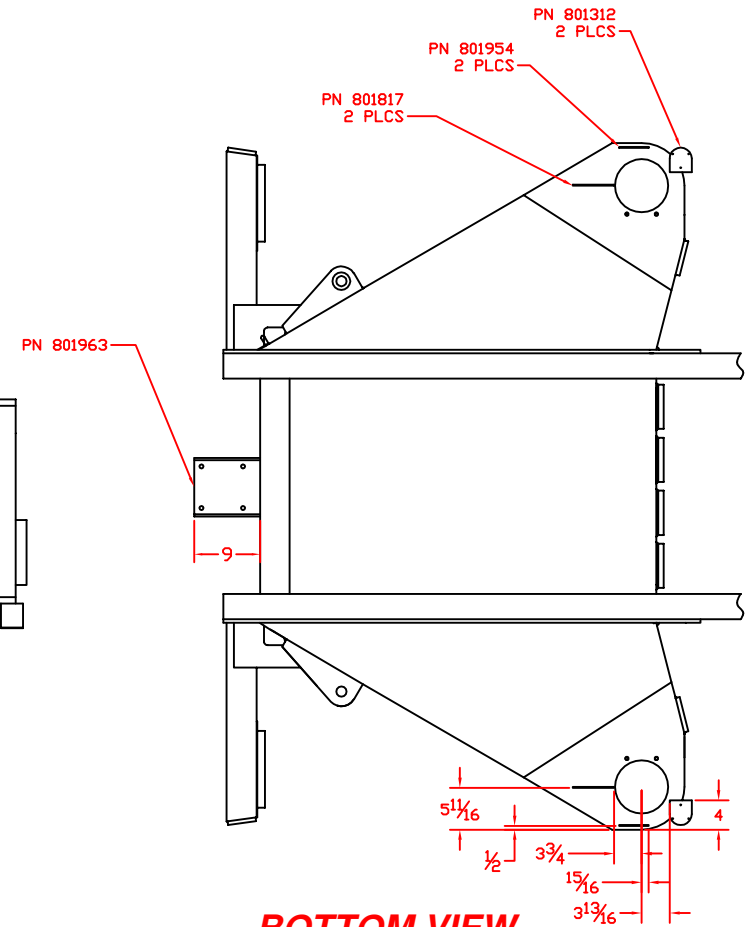
BOTTOM VIEW (AS MODIFIED)
