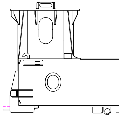
SIDE VIEW (AS MODIFIED)
