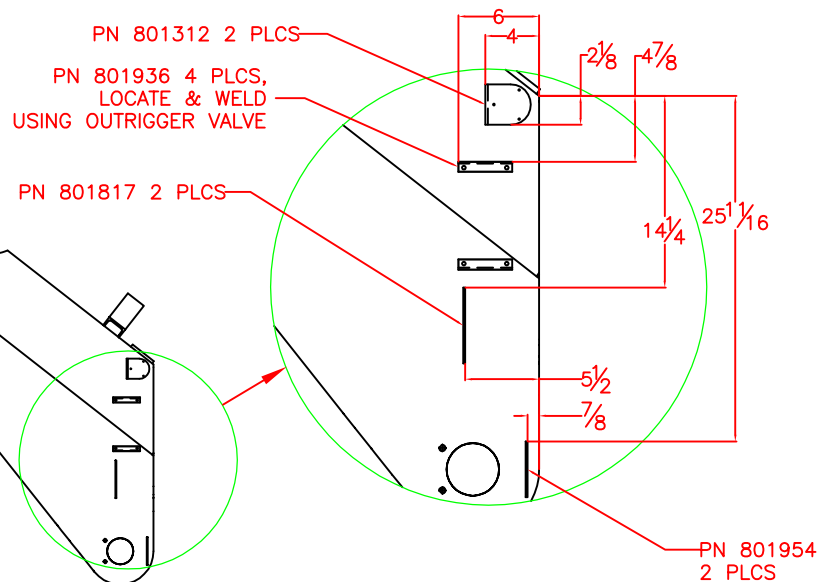
SECTION C-C
