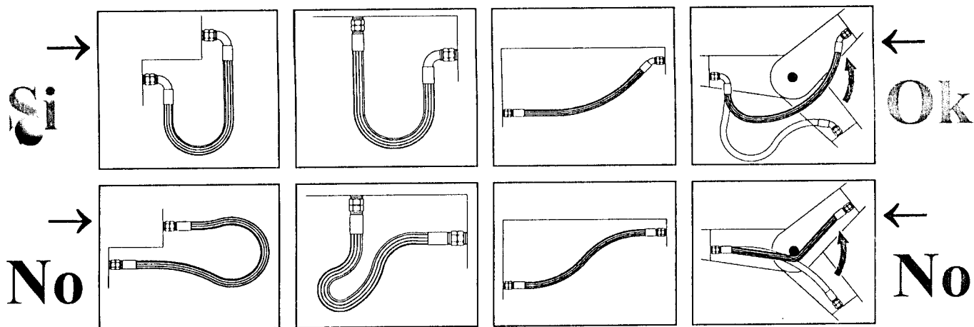
Flexible hose table
